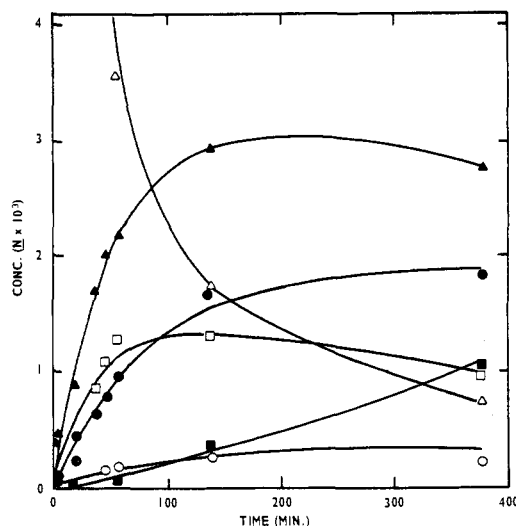
Figure 2. Products formed on irradiation of 1-iodo-8-phenylnaphthalene as a function of time: \Delta , 1-iodo-8-phenylnaphthalene ( 7 ); \blacktriangle , 1-( o -iodophenyl)naphthalene ( 1 , X = I ); \bullet , 1-phenylnaphthalene ( 2 ); \circ , fluoranthene ( 3 ); \square , 1-(2-biphenyl)naphthalene ( 4 ); \blacksquare , benzo[ g ]chrysene ( 5 ).
