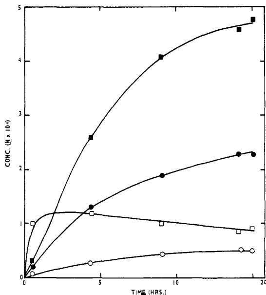
Figure 1. Products formed on irradiation of 1-( o -bromophenyl)naphthalene as a function of time: ●, 1-phenylnaphthalene (2); ○, fluoranthene (3); □, 1-(2-biphenyl)naphthalene (4); ■, benzo[ g ]chrysene (5).
